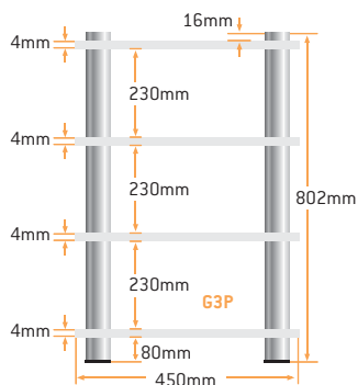
G3P - Polished gold rods shown here with clear 4mm glass and a clear 4mm storage shelf.
