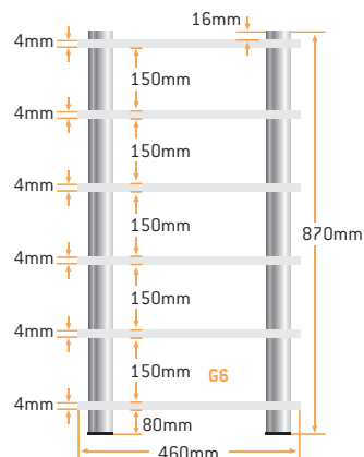
G6B - Stainless steel rods shown here with smoked 4mm glass.
