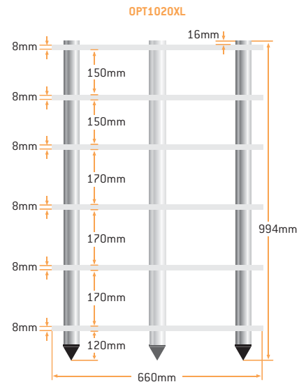
OPT1020XL - Satin black rods shown here with excel smoked 8mm glass.
