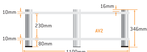
AV2B - Polished chrome rods shown here with corner smoked 10mm glass.
