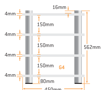
G4TT - Polished gold rods shown here with clear 4mm glass and a 4mm clear turntable shelf.
